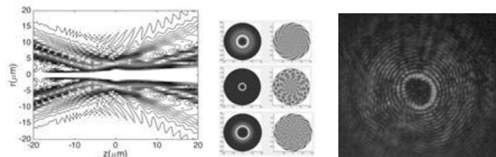
Fig.2 Intensity distribution inside the focal region.
