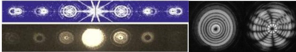
Fig.1 Pattern of diffracted LG beam from a CGH mask, analytical (top) and experimental results(lower).
