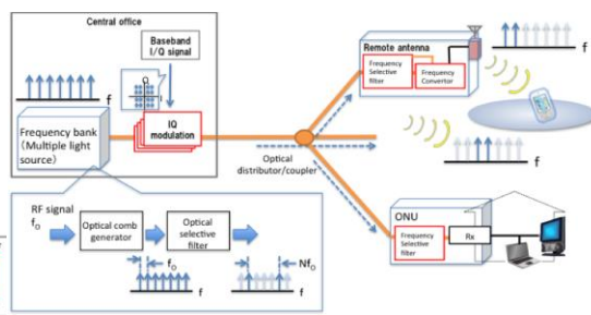
Fig.2 Proposed optical and wireless converged access network configuration
