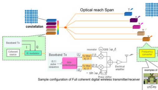
Fig.1 Fully coherent optical transmission system
