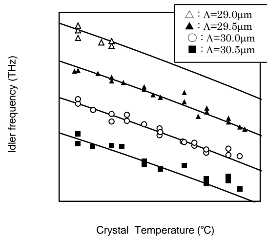
Fig 2. Temperature tuning curves for the idler frequency of QPM /OPO pumped at 1.55 \mu\text{m} . The experimental points are quoted from Ref.4.
